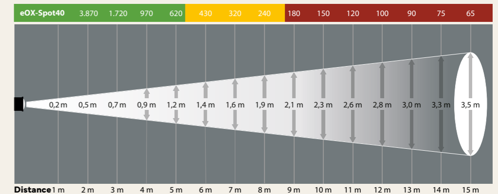
eOX SPOT 40 Illuminance [lux]
