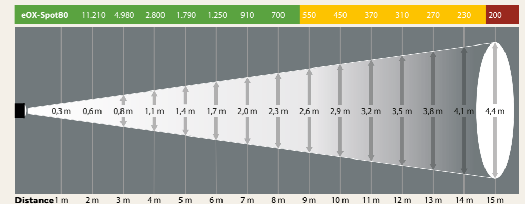
eOX-SPOT 80 Illuminance [lux]
